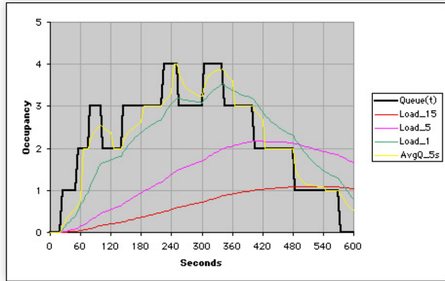
Figure 3: All three load average curves.
